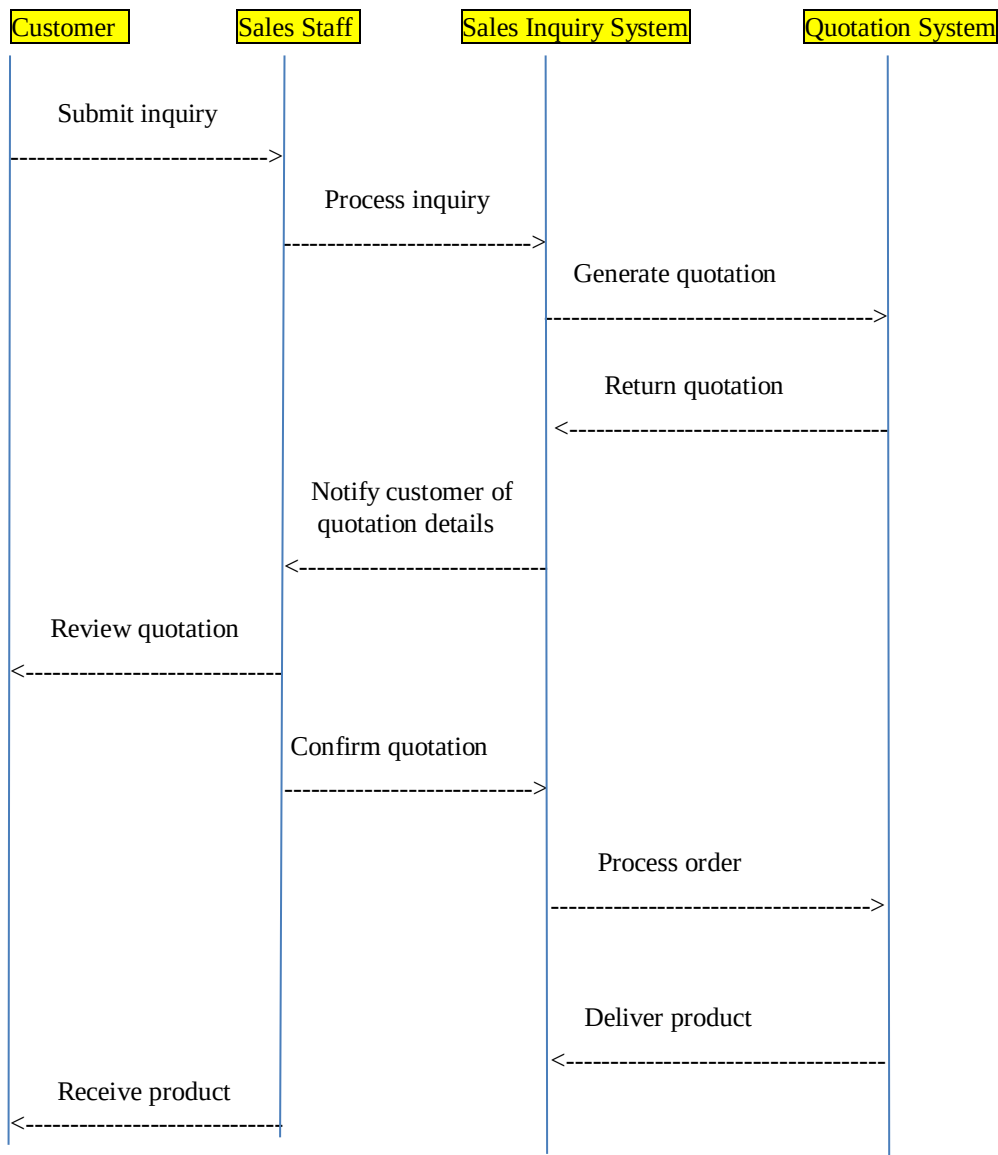
Fig 7.2.2 – Sequence Diagram
