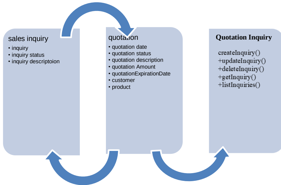
Fig 7.2.3-Class Diagram
